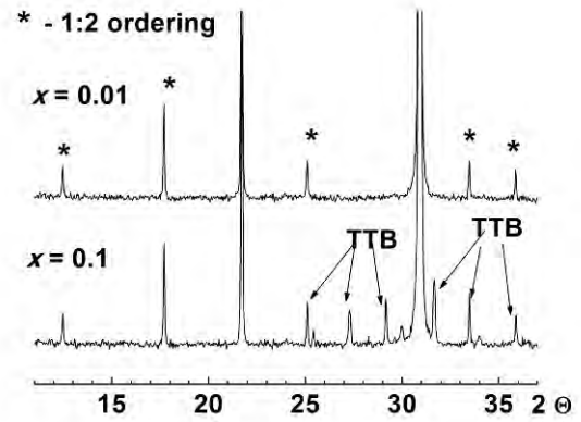
Fig. 5. XRD patterns collected on the crushed powder of the samples Ba_{1-x}(Mg_{1/3}Nb_{2/3})O_{3-x} sintered at 1550 °C for 8 hours. TTB- Ba_9MgNb_{14}O_{45}
