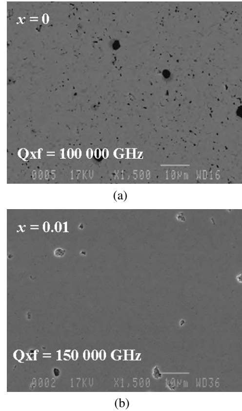
Fig. 10. SEM microphotographs of the polished surface of the ceramics Ba_{1-x}(Mg_{1/3}Nb_{2/3})O_{3-x} sintered at 1550^\circ C for 8 hours; (a) x = 0 ; (b) x = 0.01 .
